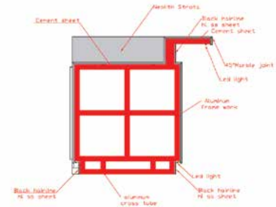
SECTION DRAWING
