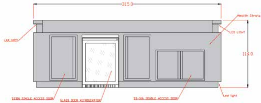
ELEVATION DRAWING
